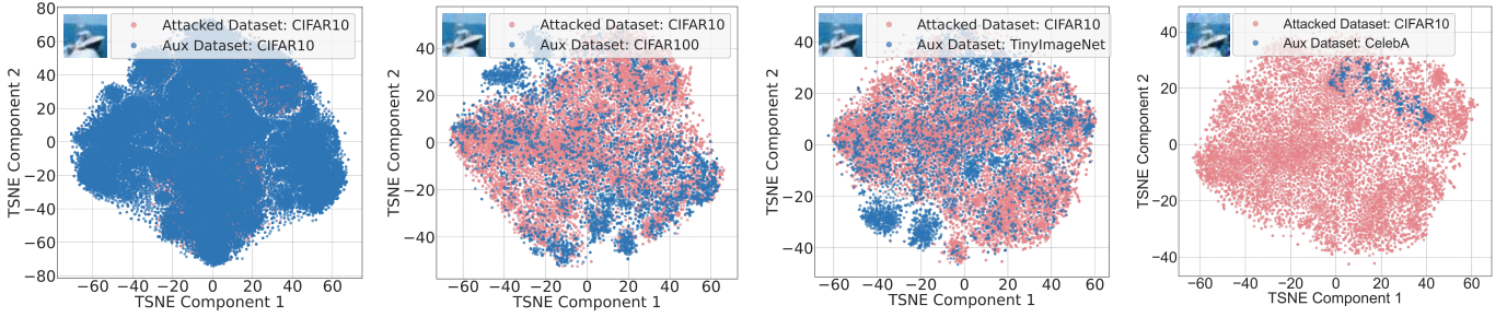
Fig. 7. Visualization of distributional differences between auxiliary and target datasets and IG reconstruction results on EGGV-poisoned models using each auxiliary dataset.
