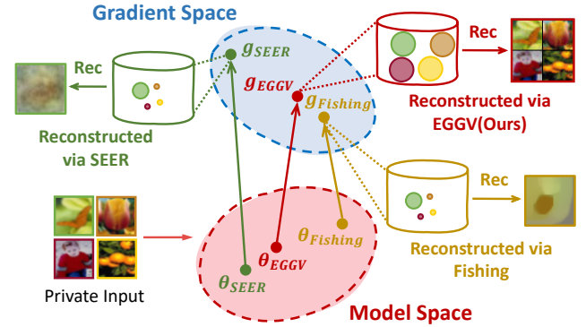
Fig. 1. Illustration of the core principles and reconstruction outcomes of Fishing [14], SEER [15], and EGGV (Ours). Each cylinder denotes the gradient space of a batch, where each inner circle represents the features of each sample contained in the average gradient, with a larger radius indicating more features contained in the averaged gradient for that sample. Existing AGLAs amplify a few samples while suppressing others, leading to partial recovery. In contrast, EGGV (Ours) uniformly enhances the feature of all samples in the gradient, enabling full-batch reconstruction.
