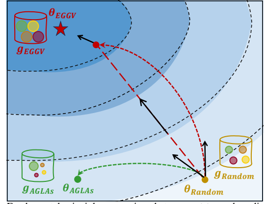
Fig. 2. Fundamental principle comparison between EGGV and gradient-biased AGLAs.
