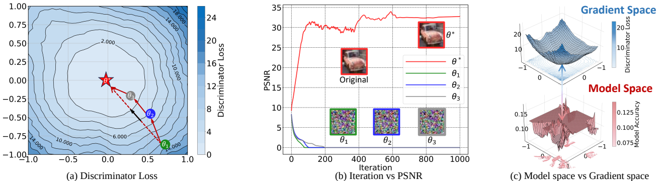
Fig. 6. Figure (a): Contour map of the discriminator loss landscape across 441 model parameters generated by shifting \theta^* along two random directions. The map marks the selected points \theta_1 , \theta_2 , \theta_3 , and \theta^* . Figure (b): PSNR curves from IG attacks on a ResNet18 model at \theta_1 , \theta_2 , \theta_3 , and \theta^* , demonstrating that \theta^* achieves the best reconstruction quality. Figure (c): 3D surface plots of the discriminator loss (top) and model accuracy (bottom) for the same 441 model parameters shifted \theta^* along two random directions, illustrating the relationship between gradient vulnerability and model accuracy across the parameter space.
