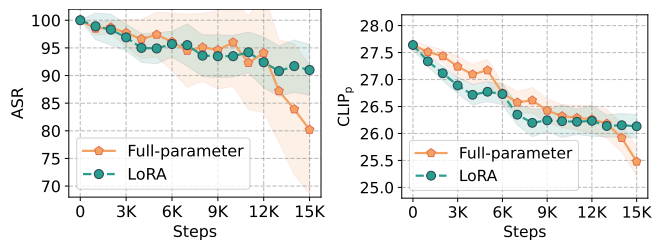
Figure 9: ASR (left) and \text{CLIP}_p (right) values with varying further fine-tuning iterations.
