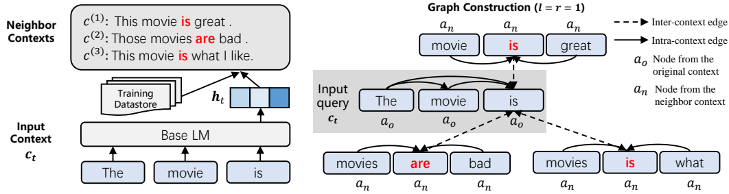
Figure 1: An overview of the proposed GNN-LM model pipeline. Left : Given an input context c_t = (w_1, \dots, w_{t-1}) (here the context is “The movie is”), a base LM model encodes it into a high-dimensional representation h_t , which is then used to query the training datastore to retrieve the nearest contexts along with the visited tokens (marked in red). Right : The tokens in the input context and the retrieved tokens comprise a graph and are viewed as two types of nodes: nodes from the original text and nodes from the neighbor text. Inter-context edges link tokens within the same input, and intra-context edges link tokens from the retrieved contexts to the original context. After modeling the graph as a whole with GNNs, we use the updated representation of w_{t-1} (token “is” in this example) to compute the likelihood of the next token.
